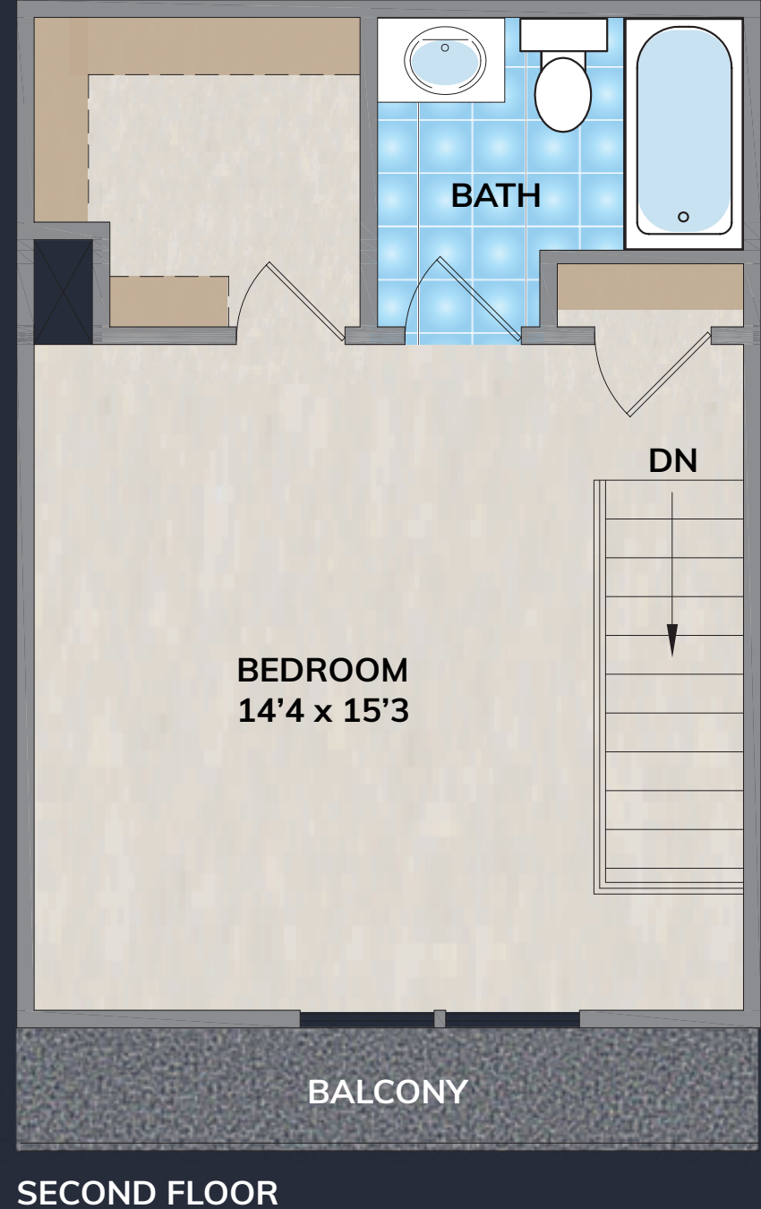
BOARDWALK WEST APARTMENTS UNIT TYPE "D", 1 BEDROOM, 1 1/2 BATH 697 Sq. Ft.
